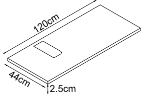
Technical Drawing :
