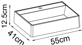
Technical Drawing :
