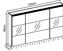
Technical Drawing :
