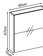
Technical Drawing :
