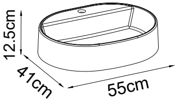
Technical Drawing :
